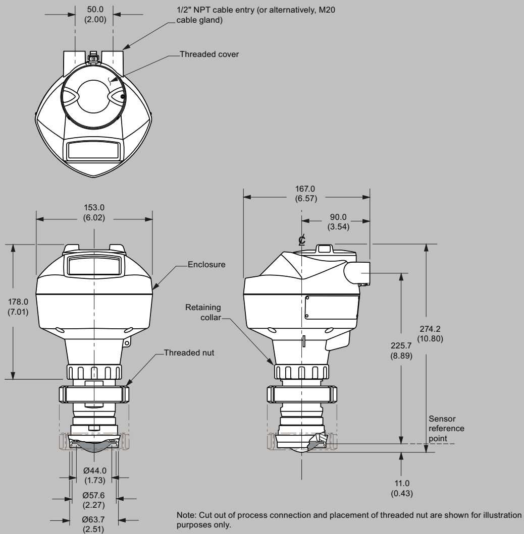
SITRANS LR250 Hygienic Encapsulated Antenna (DN 50 nozzle/slotted nut to DIN 11851), dimensions in mm (inch)
